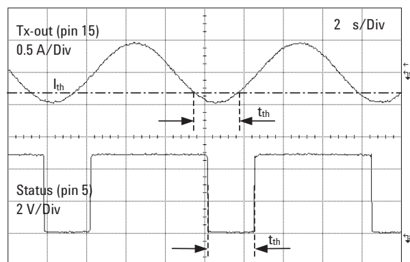
Figure 29. Transmit output load detection
